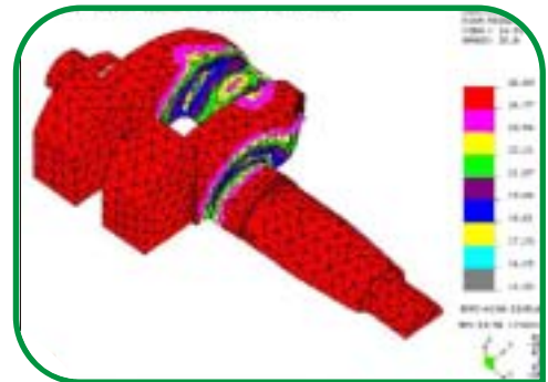
Log (Life) contours on crank shaft
